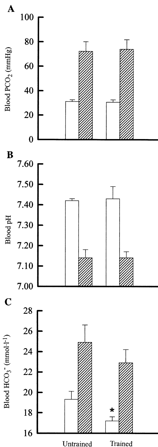
Fig. 3. Femoral arterial (open bars) and venous (hatched bars) blood PCO 2 (A), pH (B), and HCO 3 - (C) at the end of intense knee-extensor exercise in untrained and trained leg; n = 5 subjects. Values are means \pm SE. *Significantly different from untrained leg, P < 0.05 .
